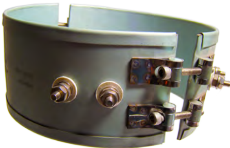
CERAMIC BAND HEATERS
